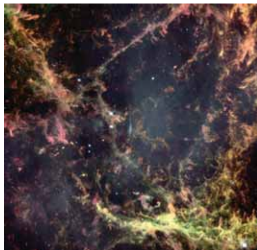
Figure 3-1: Image of wisps of gas, which are all that remain of a once mighty 15-solar-mass supergiant star that exploded thousands of years ago
