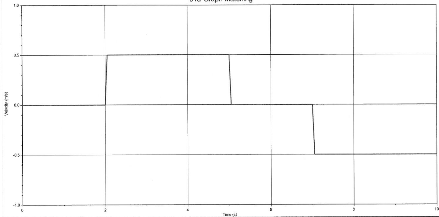
01d-Graph Matching
