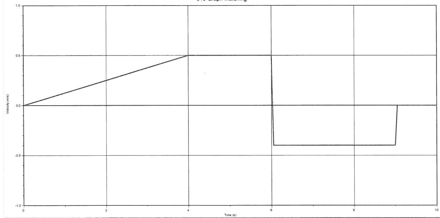
01e-Graph Matching
